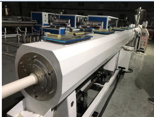
Vacuum cooling tank
