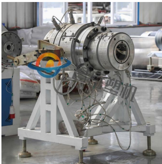
PVC pipe mould PVC pipe size: 50-200 mm heater: ceramic heater
